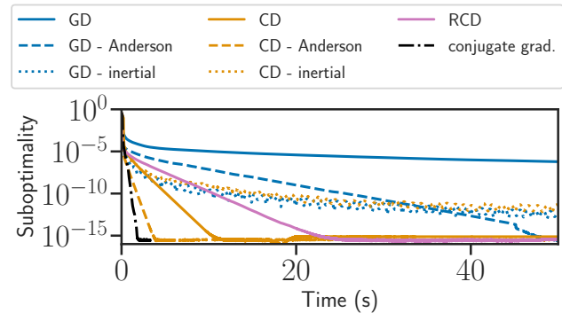
Figure 1: Suboptimality along time for a quadratic problem on the 5000 first features of the rcv1 dataset. GD: gradient descent, (R)CD: (randomized) coordinate descent.
