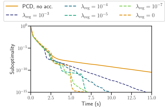
Figure 6: Influence of \lambda_{\text{reg}} , sparse logistic regression, rcv1 . Influence of the regularization amount when solving a sparse logistic regression using Anderson extrapolation with proximal coordinate descent (PCD) on the rcv1 dataset, K = 5 , \lambda = \lambda_{\text{max}}/30 .
